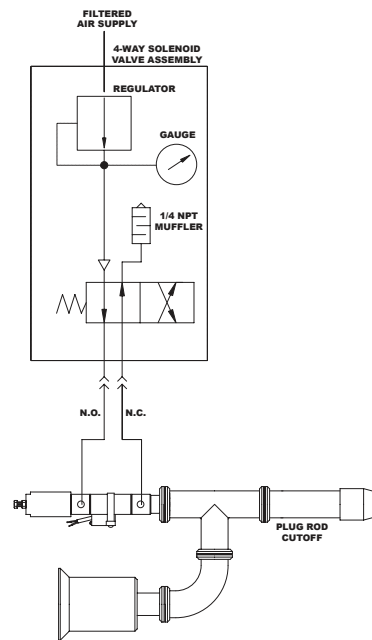
Rod Cutoff Air Schematic
